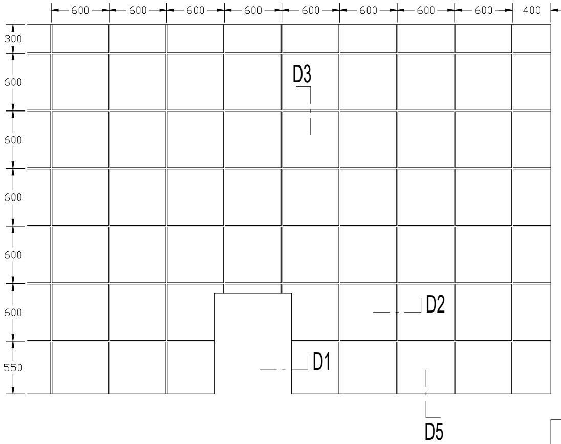
CEILING TILES LAY-OUT
